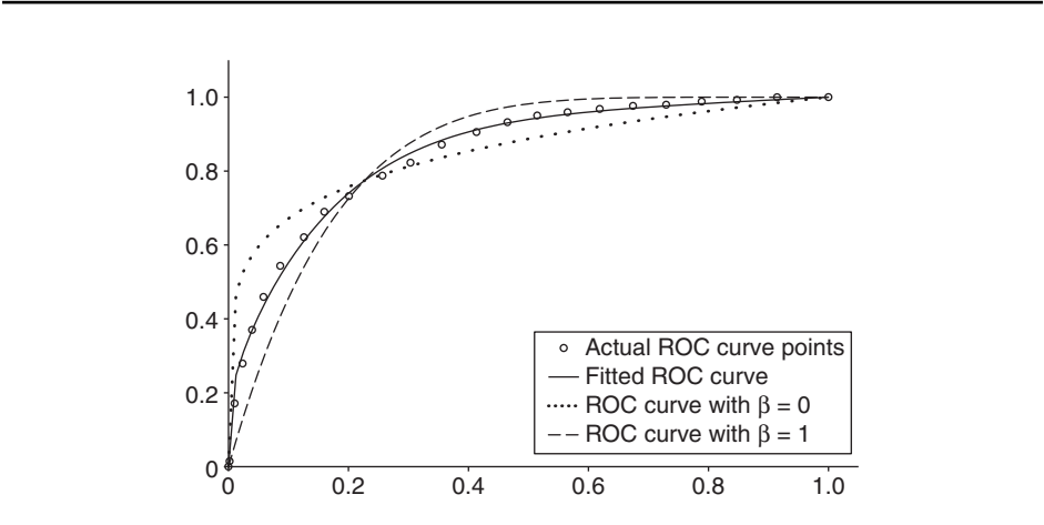
FIGURE 8 A curve fitted to the empirical ROC curve found in Wójcicki and Migut (2010).
