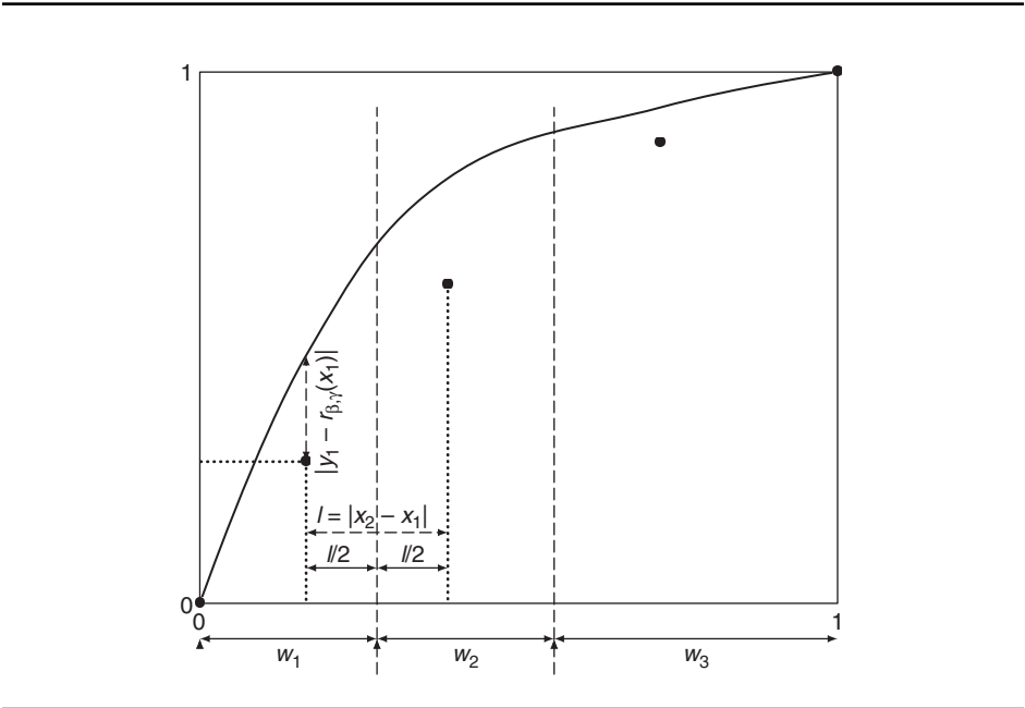
FIGURE 5 Setting weights for the “bobyqa” objective function.
