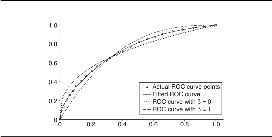
FIGURE 7 A curve fitted to more data points read from the Lorenz curve in Řezáč and Řezáč (2011).
