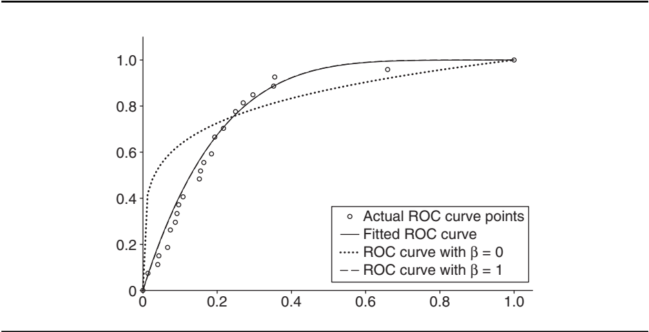
FIGURE 11 A curve fitted to the empirical data on a model for individual entrepreneurs from Miyamoto (2014).
